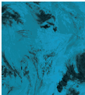
Artificial Intelligence
